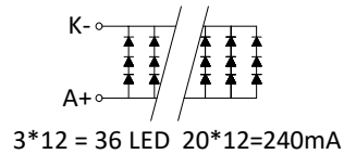
Internal Circuit Diagram
