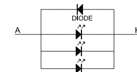
BLACKLIGHT CIRCUIT
